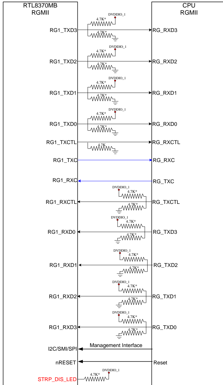
Figure 29. Signal Diagram of RGMII Mode of the Extension GMAC1
