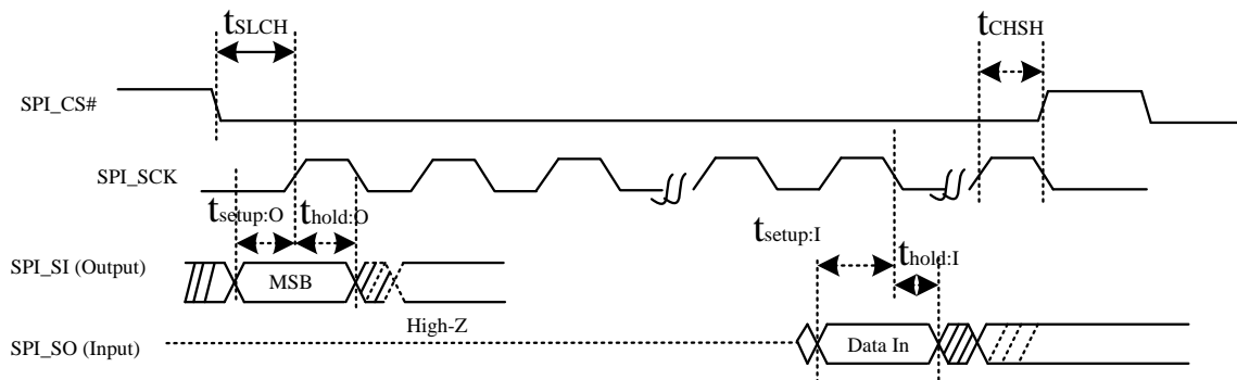
Figure 48. SPI FLASH Timing Characteristics
