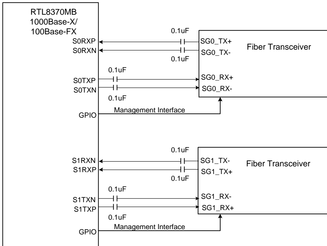
Figure 44. Signal Diagram of 1000Base-X/100Base-FX Mode of the Extension GMAC1/GMAC2
