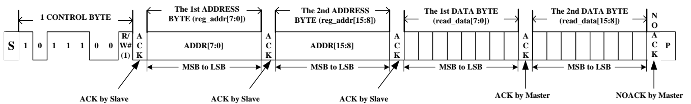
Figure 23. I2C-Like Slave Interface Read Command
