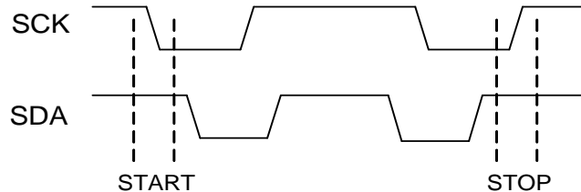
Figure 17. I2C Start and Stop Command
