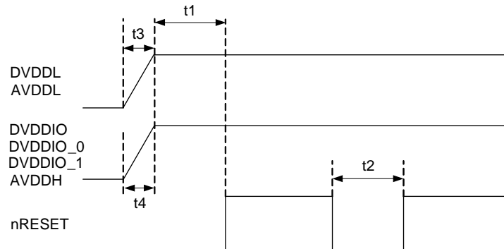
Figure 73. Power and Reset Characteristics
