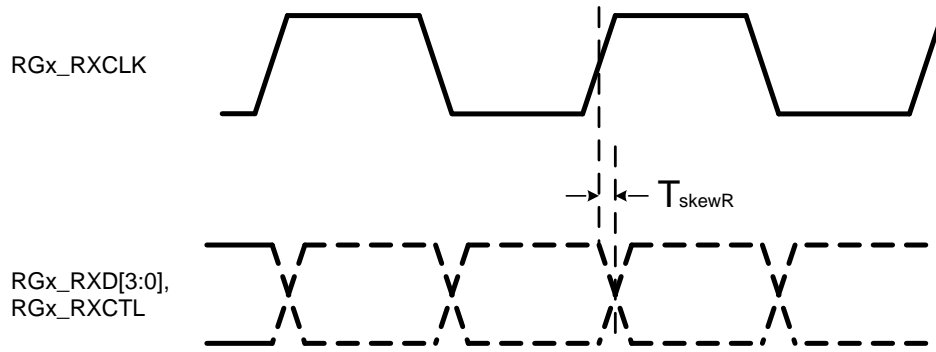
Figure 56. RGMII Input Timing Characteristics (RGx_RXCLK_DELAY=2ns)
