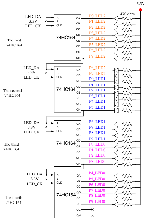
Figure 12. RTL8370MB+74HC164 Serial LED Connection Diagram (per-port three single-color LED)
