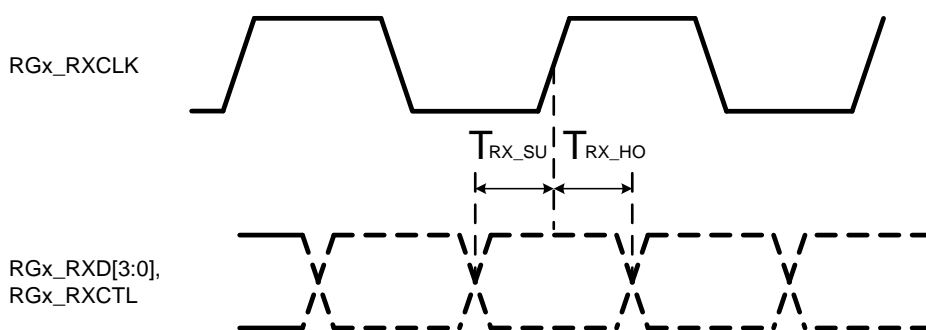
Figure 55. RGMII Input Timing Characteristics (RGx_RXCLK_DELAY=0)
