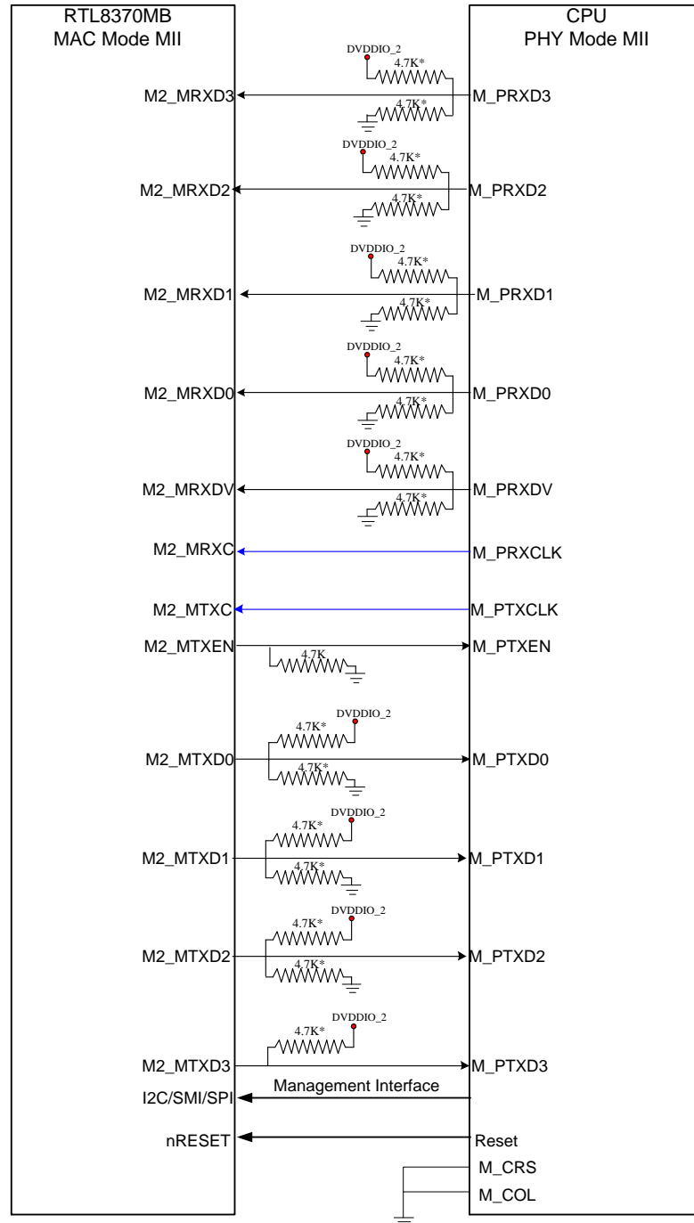
Figure 34. Signal Diagram of MII MAC Mode of the Extension GMAC2
