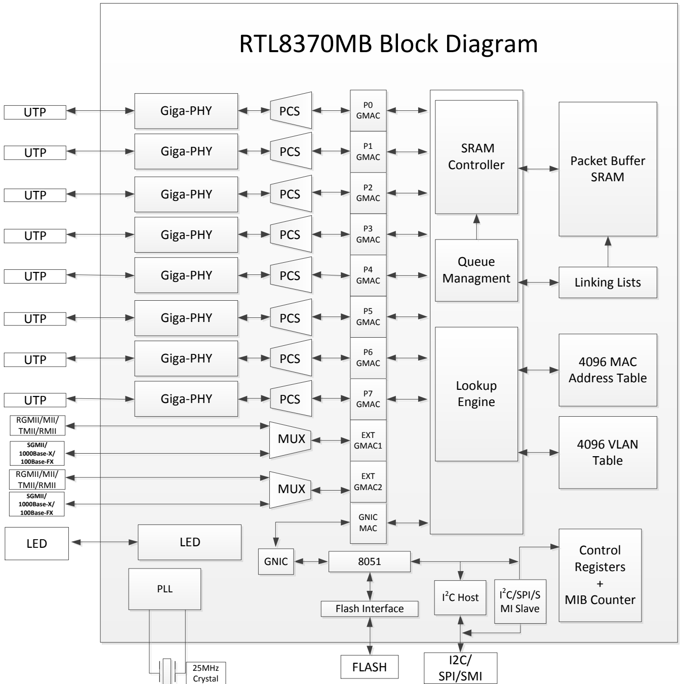
Figure 1 Block Diagram of RTL8370MB
