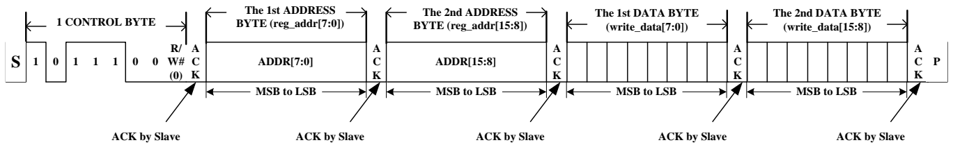
Figure 22. I2C-Like Slave Interface Write Command
