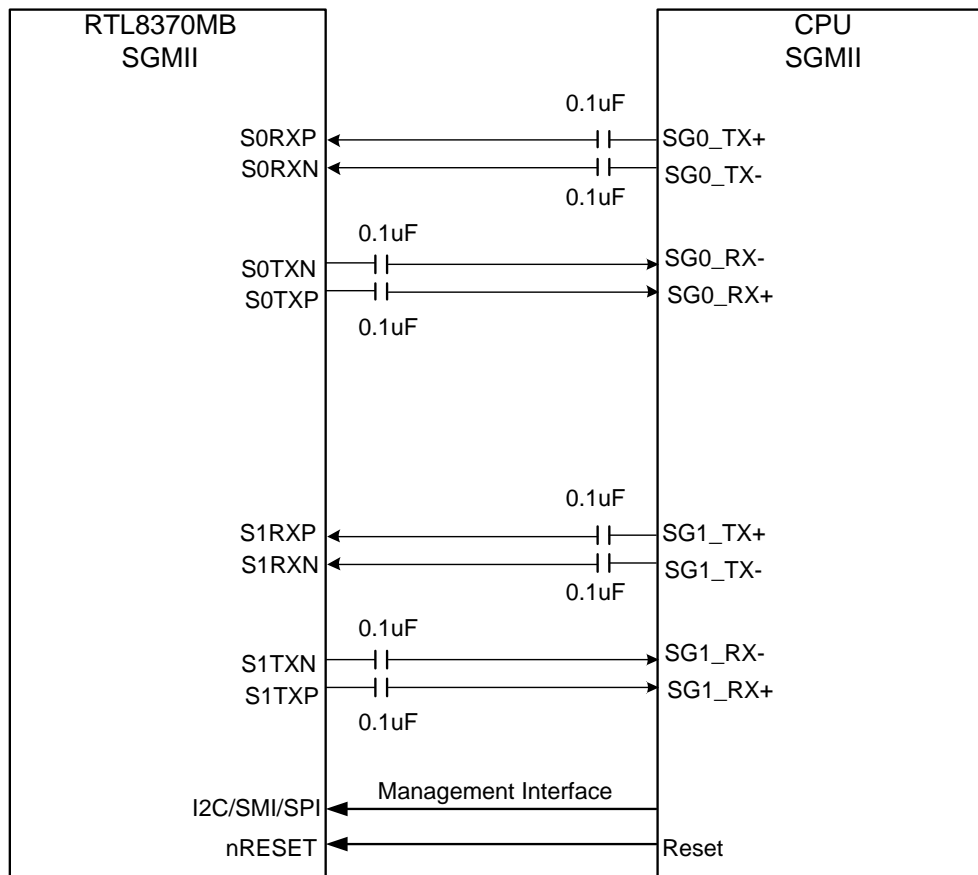
Figure 43. Signal Diagram of SGMII Mode of the Extension GMAC1 & GMAC2
