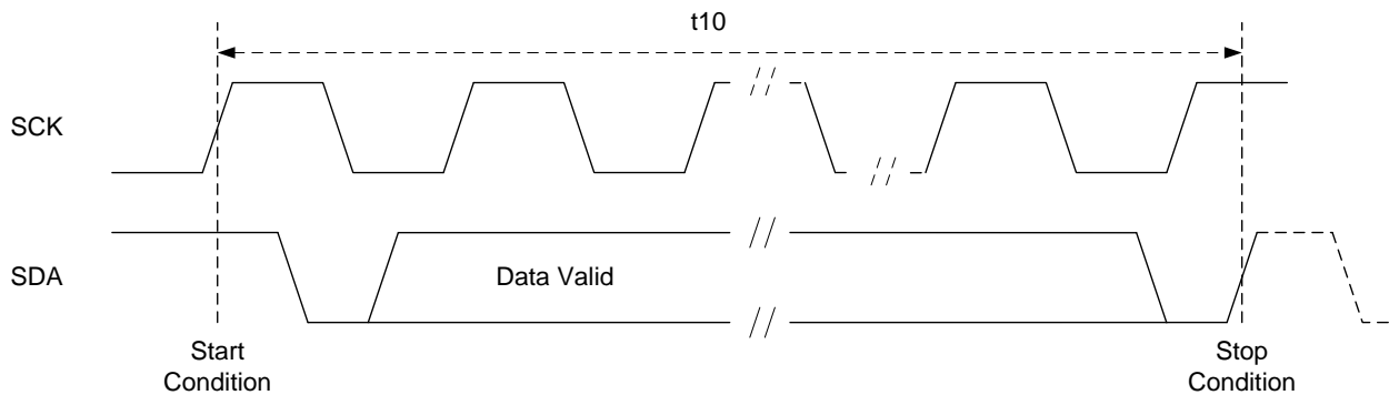
Figure 47. Master I2C for EEPROM Auto-load Timing
