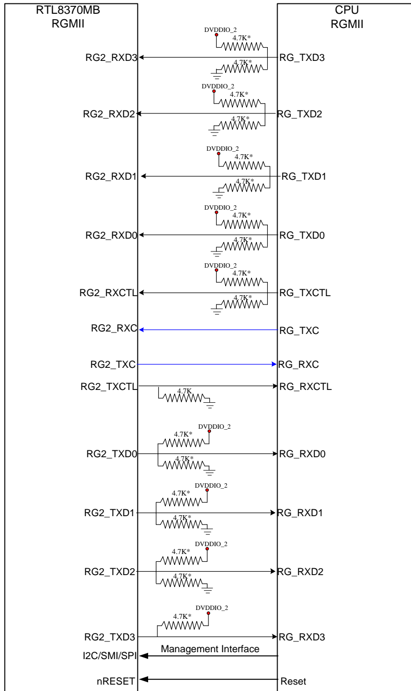
Figure 30. Signal Diagram of RGMII Mode of the Extension GMAC2
