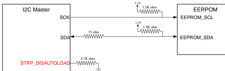
Figure 18. I2C Master for EEPROM Auto-load Interface Connection Example
