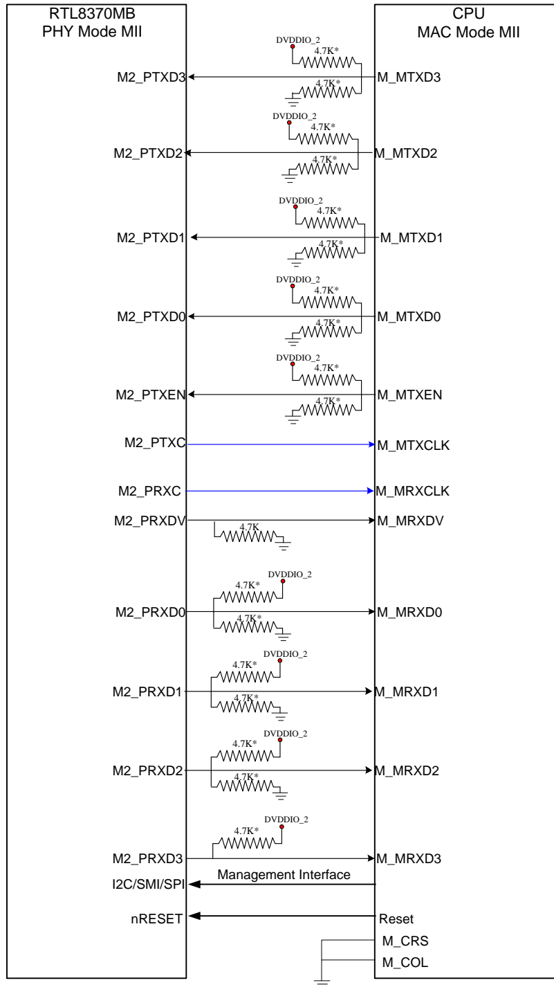
Figure 33. Signal Diagram of MII PHY Mode of the Extension GMAC2
