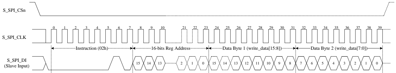
Figure 26. Slave SPI for External CPU Access Write Command
