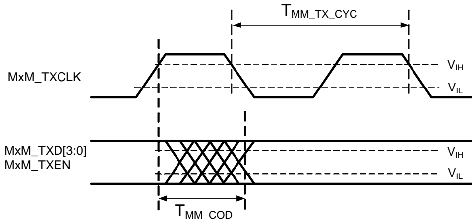
Figure 57. MII MAC Mode Clock to Data Output Delay Timing
