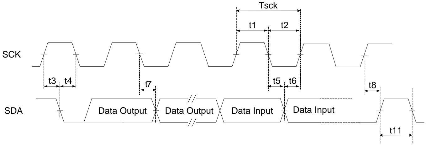
Figure 45. Master I2C for EEPROM Auto-load Timing Characteristics
