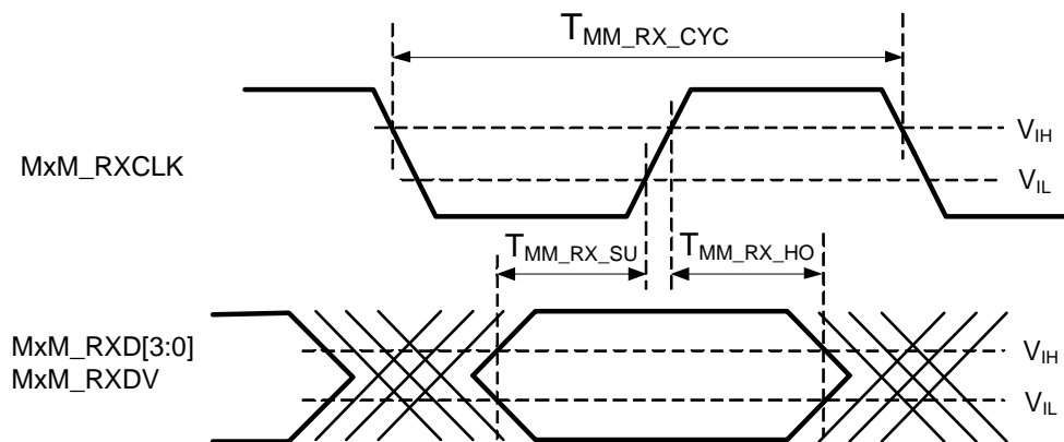
Figure 58. MII MAC Mode Input Timing
