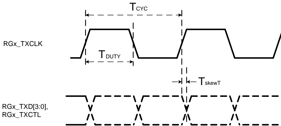
Figure 53. RGMII Output Timing Characteristics (RGx_TXCLK_DELAY=0)
