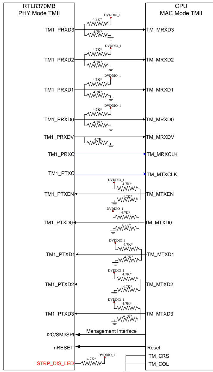
Figure 35. Signal Diagram of TMII PHY Mode of the Extension GMAC1
