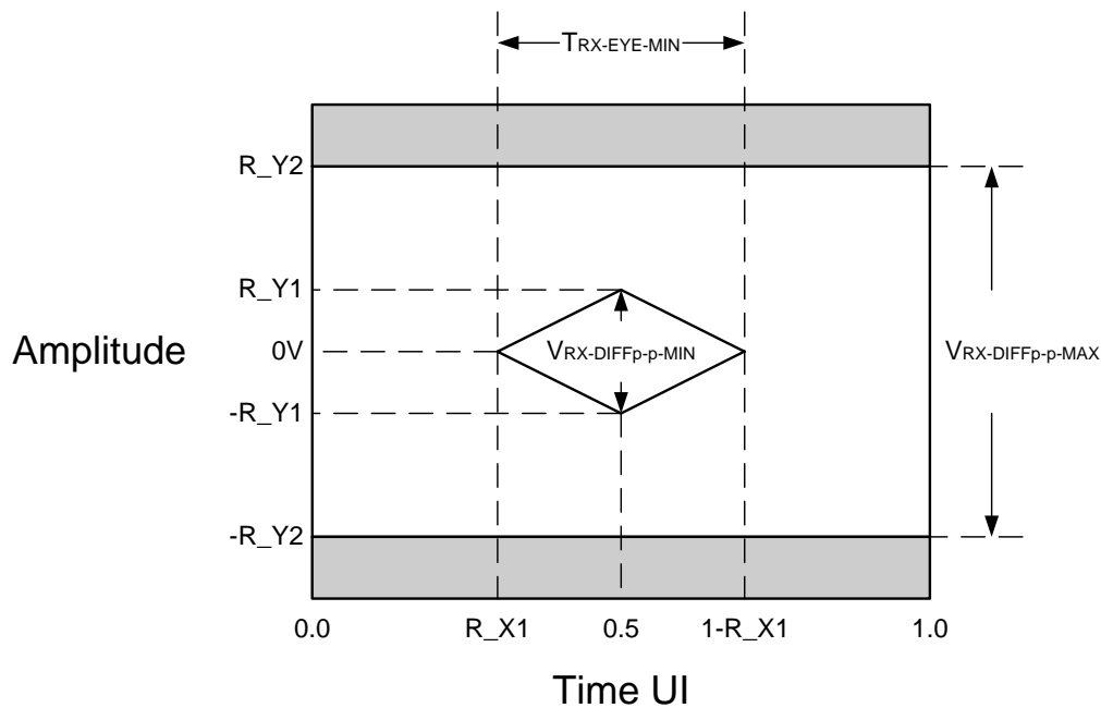
Figure 72. 1000Base-X/100Base-FX Differential Receiver Eye Diagram
