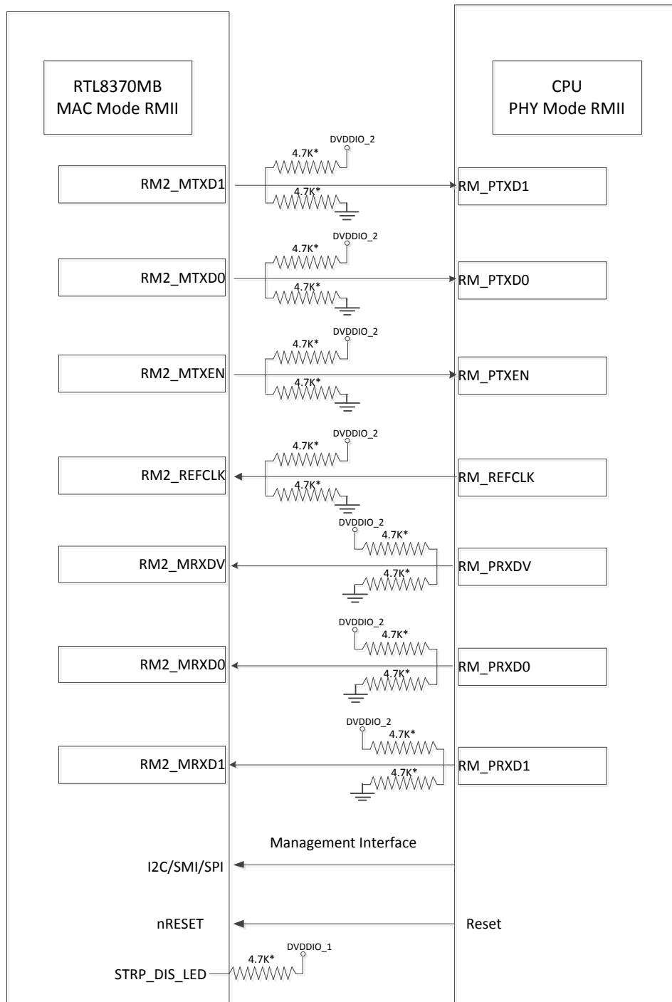
Figure 42. Signal Diagram of RMII MAC Mode of the Extension GMAC2
