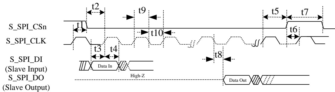
Figure 52. Slave SPI for External CPU Access Interface Timing Characteristics
