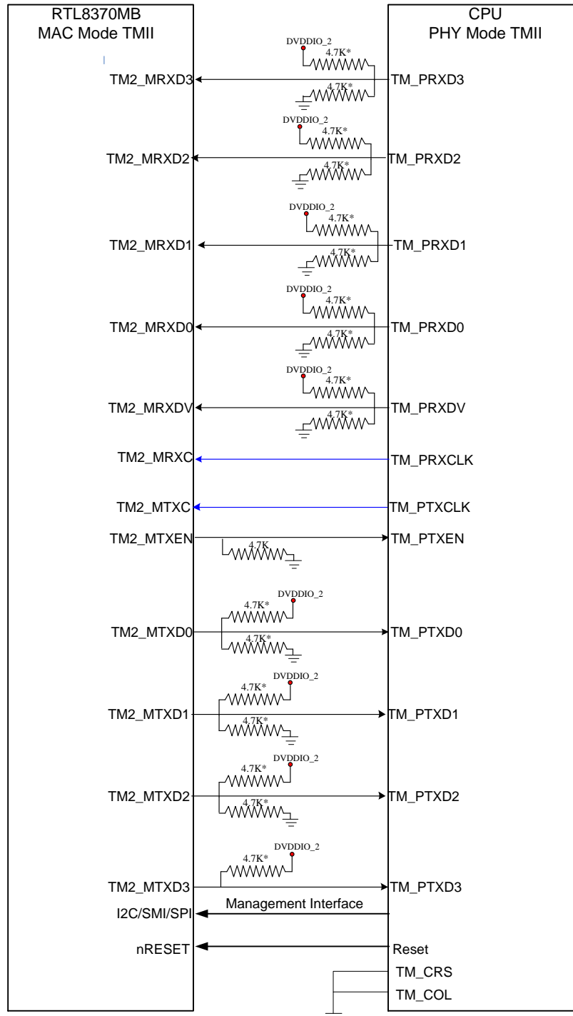
Figure 38. Signal Diagram of TMII MAC Mode of the Extension GMAC2
