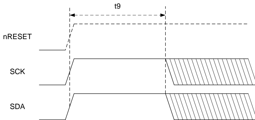
Figure 46. Master I2C for EEPROM Auto-load Power on Timing
