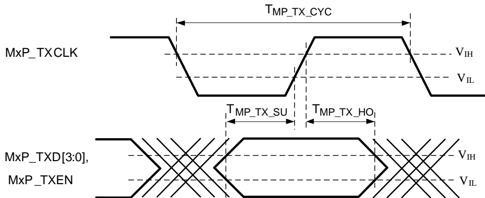
Figure 60. MII PHY Mode Input Timing
