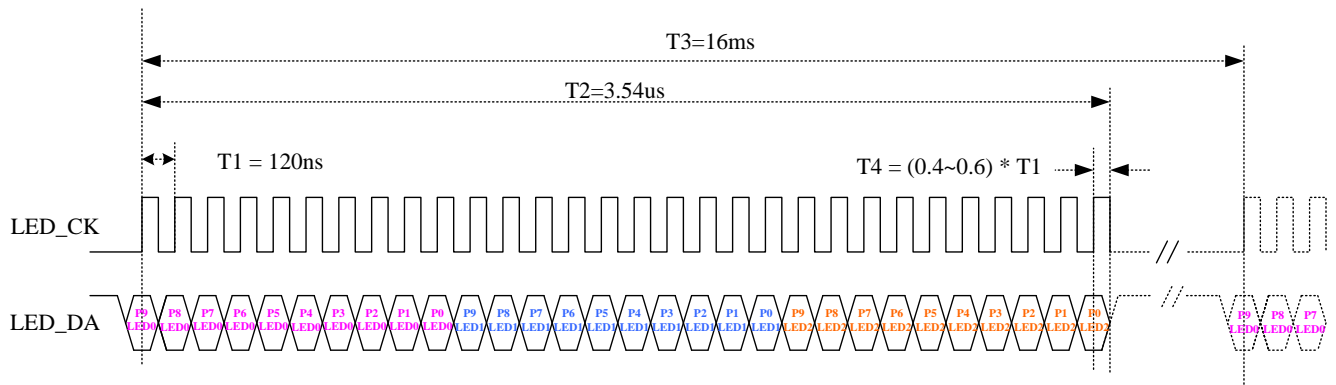
Figure 11. RTL8370MB serial led mode shift sequence (per-port three single-color LED)
