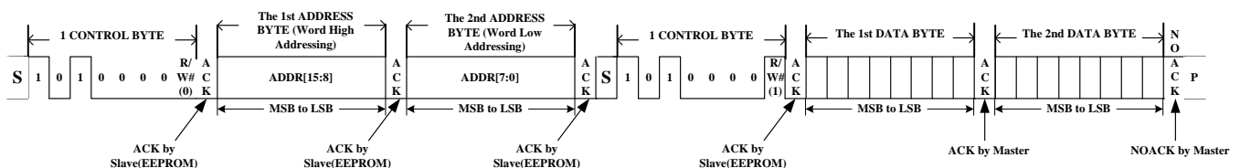
Figure 20. 16-Bit EEPROM Sequential Read
