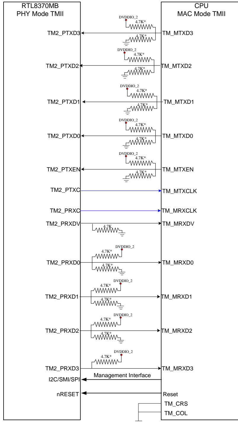
Figure 37. Signal Diagram of TMII PHY Mode of the Extension GMAC2
