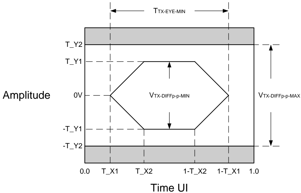
Figure 69. SGMII Differential Transmitter Eye Diagram
