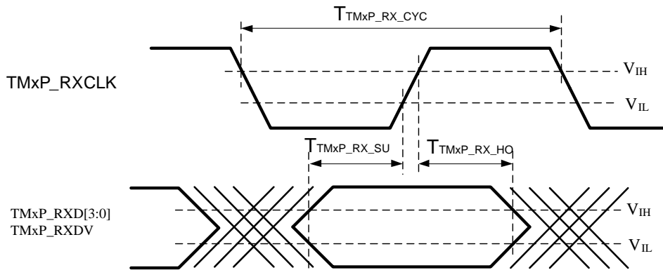
Figure 63. TMII PHY Mode Output Timing
