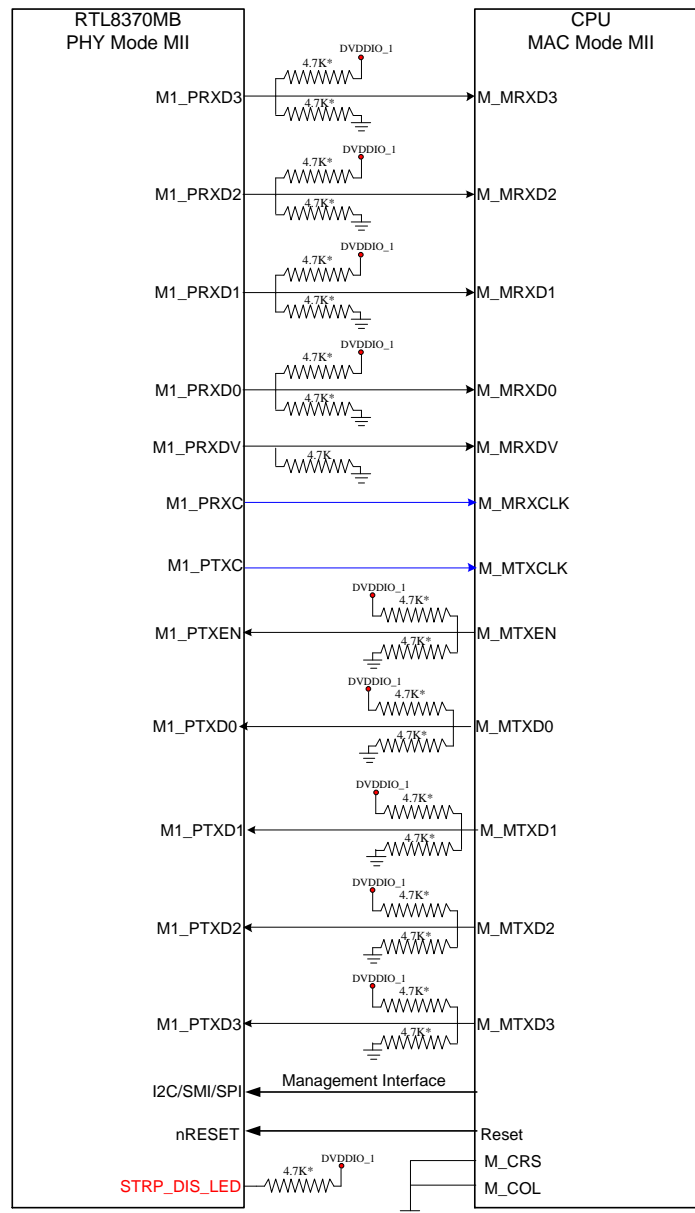
Figure 31. Signal Diagram of MII PHY Mode of the Extension GMAC1
