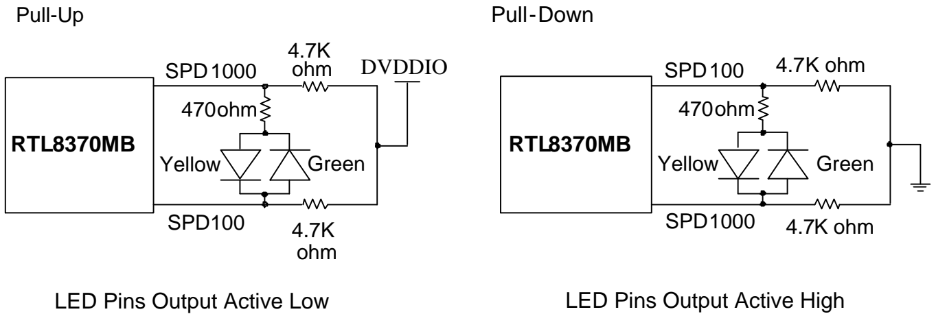
Figure 10. Pull-Up and Pull-Down of LED Pins for Bi-Color LED
