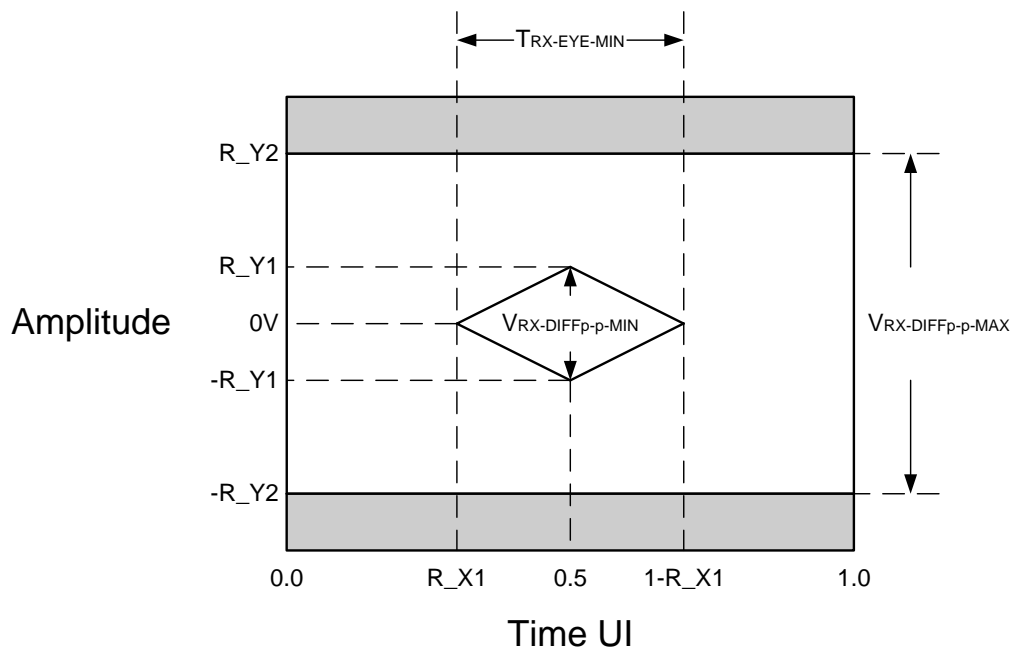
Figure 70. SGMII Differential Receiver Eye Diagram
