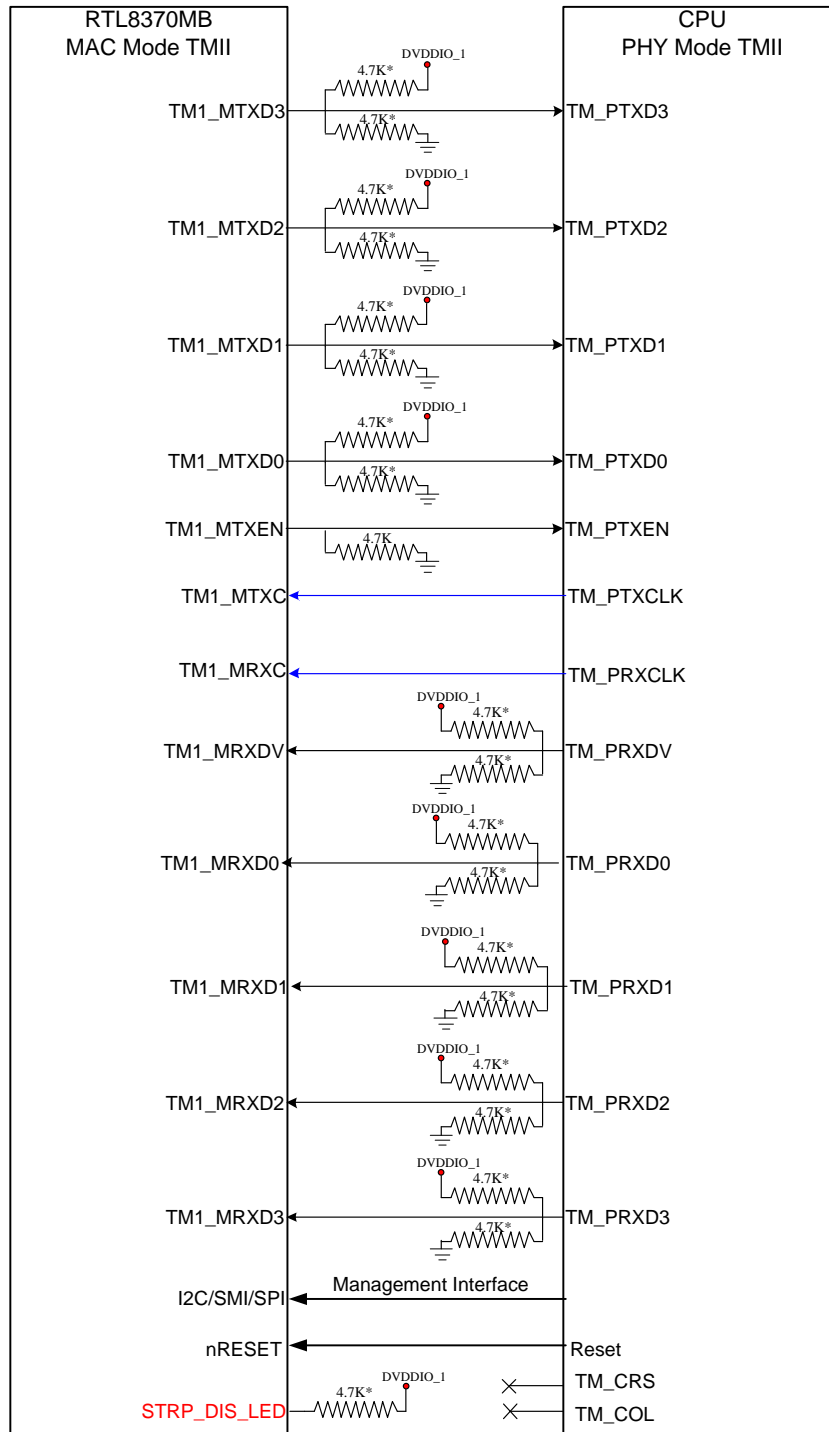
Figure 36. Signal Diagram of TMII MAC Mode of the Extension GMAC1
