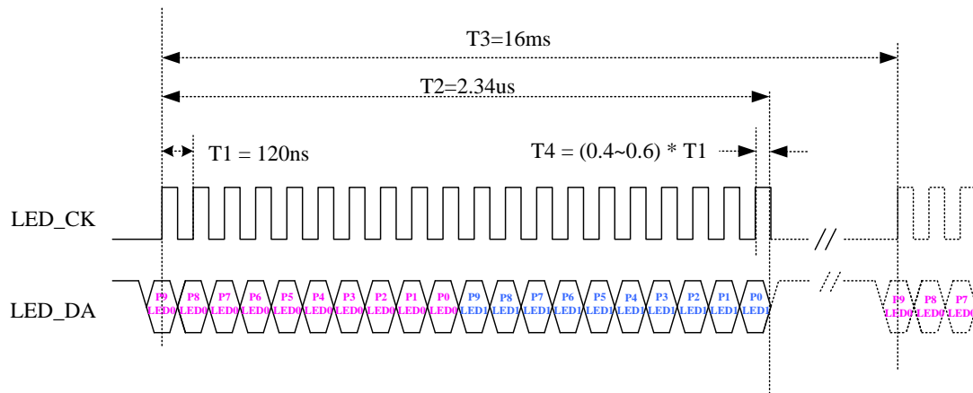
Figure 15. RTL8370MB serial led mode shift sequence (per-port two single-color LED)
