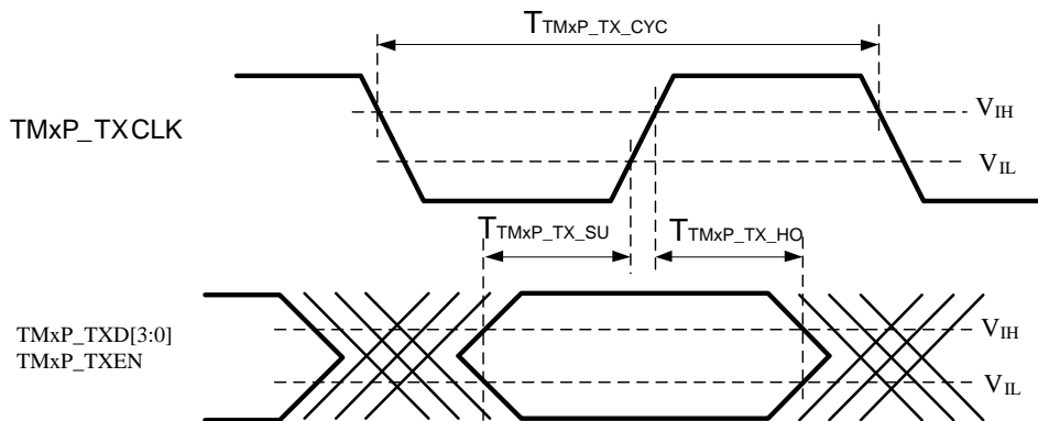
Figure 64. TMII PHY Mode Input Timing
