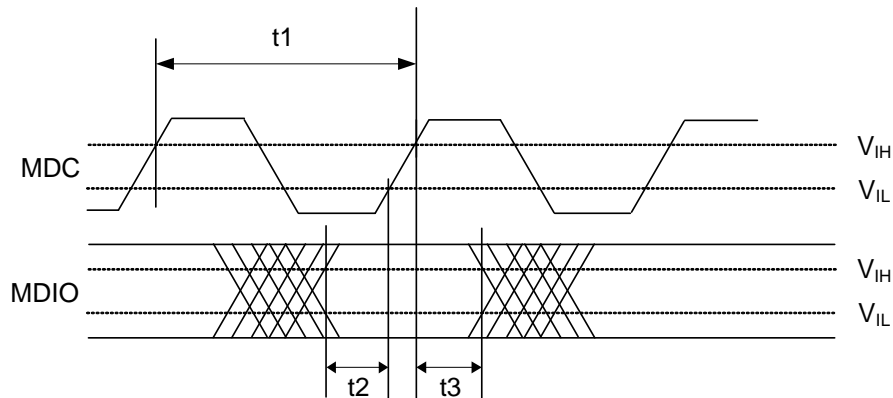
Figure 50. MDIO Sourced by Master (External CPU)
