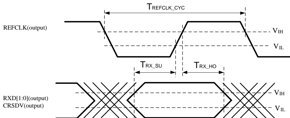
Figure 67. RMII PHY Mode Output Timing
