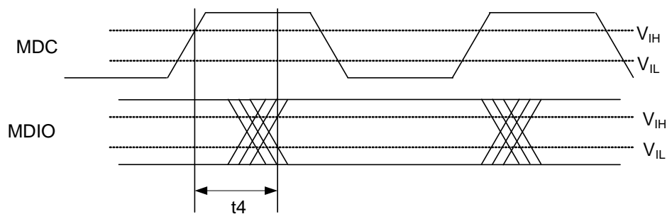
Figure 51. MDIO Sourced by Slave (RTL8370MB)
