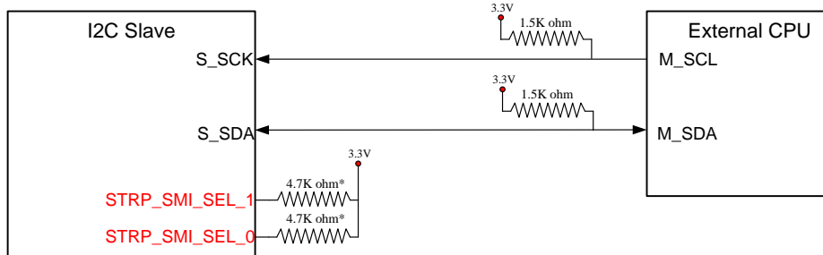
Figure 21. I2C-Like Slave for External CPU Access Interface Connection Example
