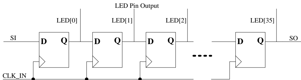
Figure 13. RTL8231 Output Data Sequence
