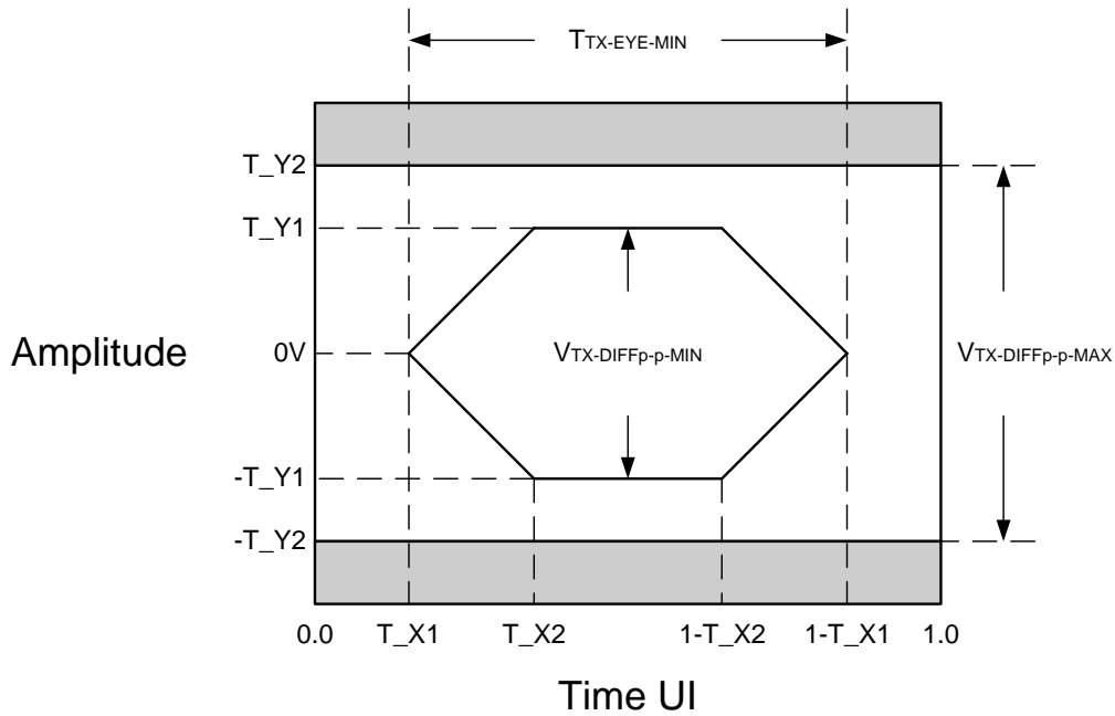
Figure 71. 1000Base-X/100Base-FX Differential Transmitter Eye Diagram
