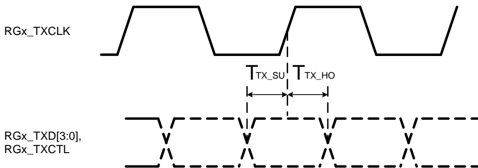
Figure 54. RGMII Output Timing Characteristics (RGx_TXCLK_DELAY=2ns)
