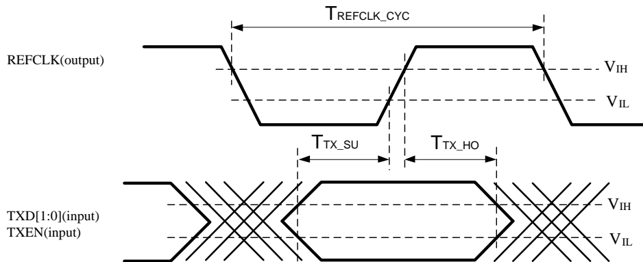
Figure 68. RMII PHY Mode Input Timing
