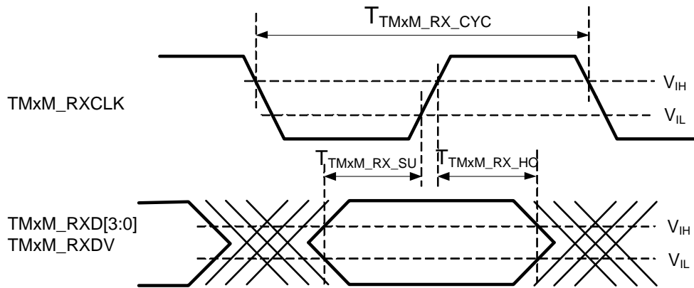
Figure 62. TMII MAC Mode Input Timing
