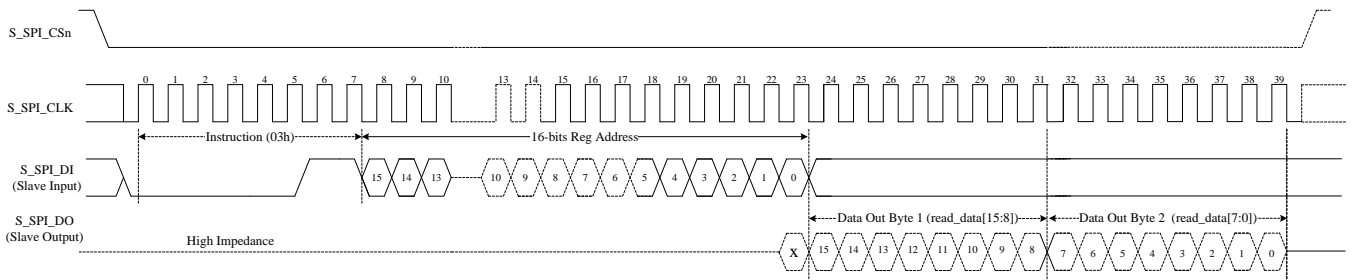
Figure 27. Slave SPI for External CPU Access Read Command
