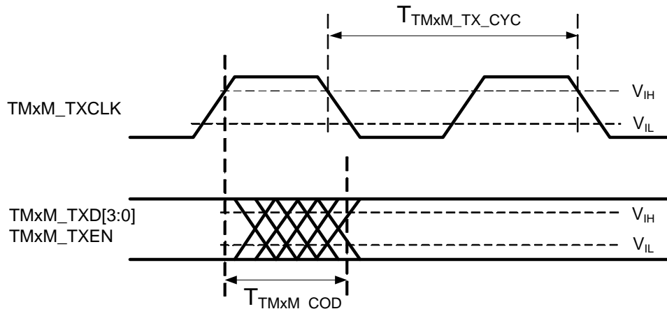
Figure 61. TMII MAC Mode Clock to Data Output Delay Timing
