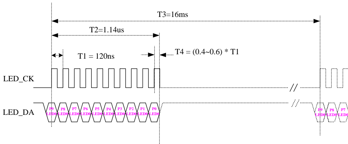
Figure 16. RTL8370MB serial led mode shift sequence (per-port one single-color LED)
