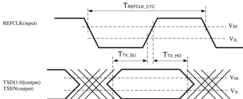
Figure 65. RMII MAC Mode Output Timing
