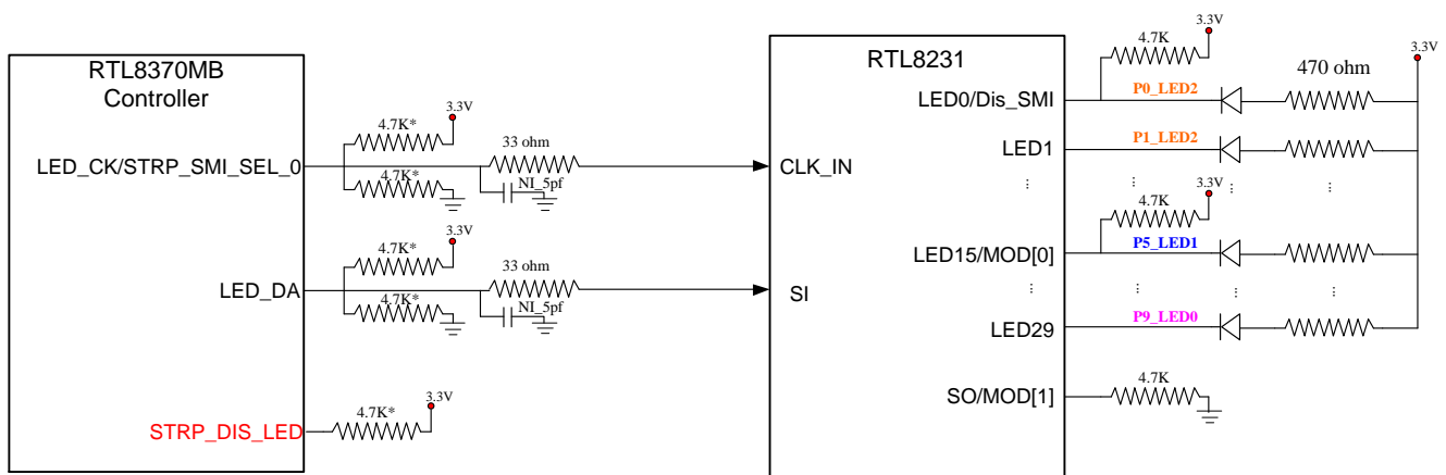
Figure 14. RTL8370MB+RTL8231 Serial LED Connection Diagram (per-port three single-color LED)
