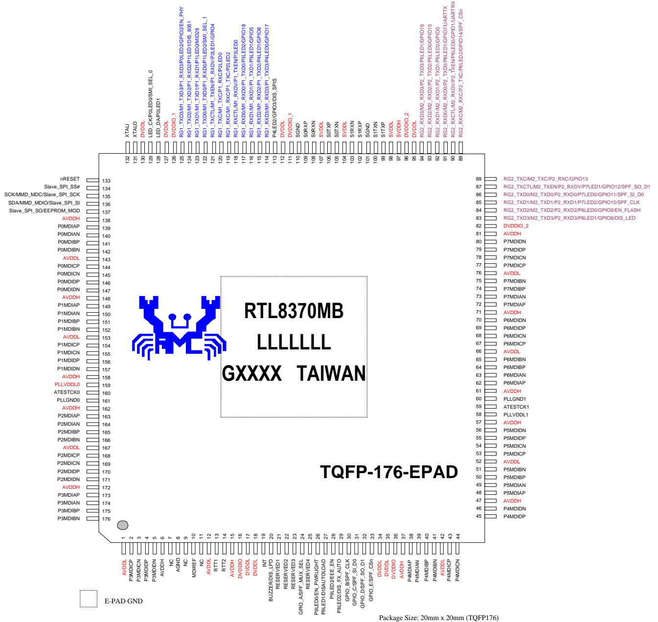
Figure 5. Pin Assignments
