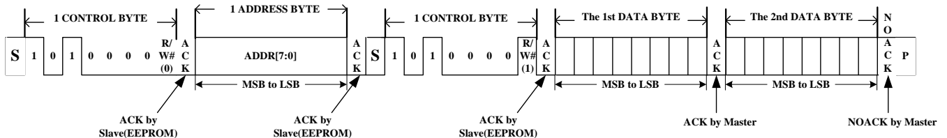
Figure 19. 8-Bit EEPROM Sequential Read
