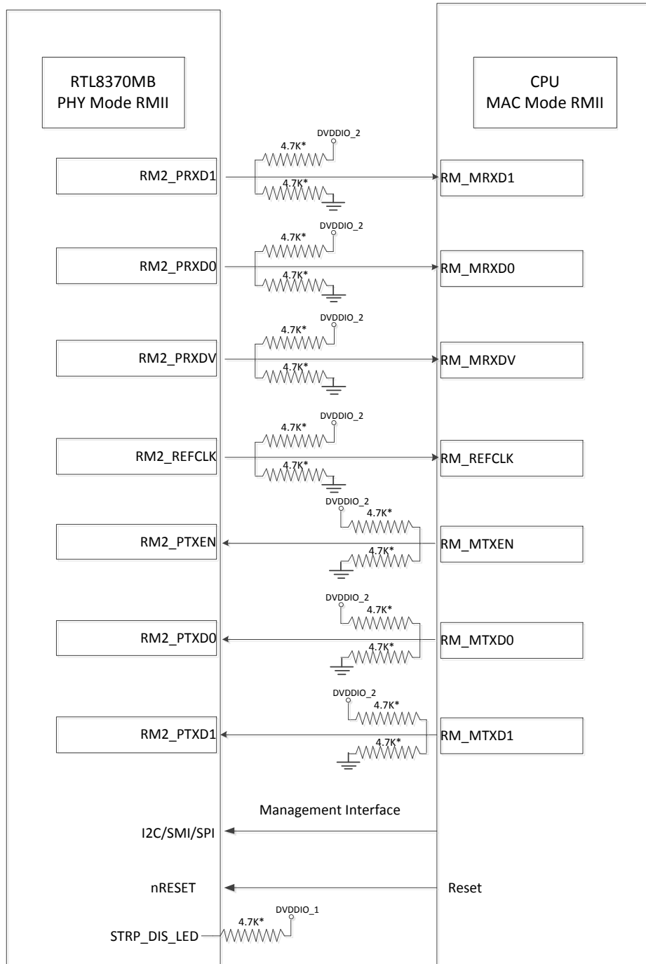
Figure 41. Signal Diagram of RMII PHY Mode of the Extension GMAC2
