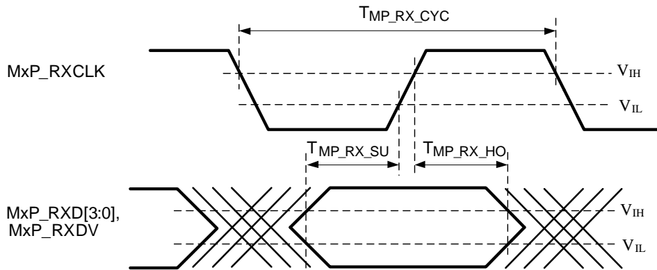
Figure 59. MII PHY Mode Output Timing
