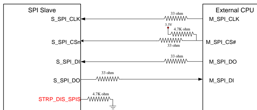
Figure 25. Slave SPI for External CPU Access Interface Connection Example
