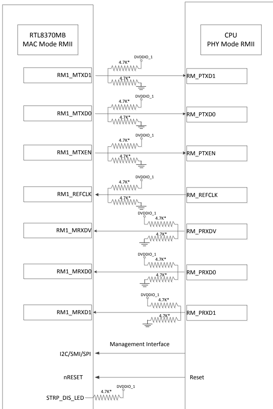
Figure 40. Signal Diagram of RMI MAC Mode of the Extension GMAC1
