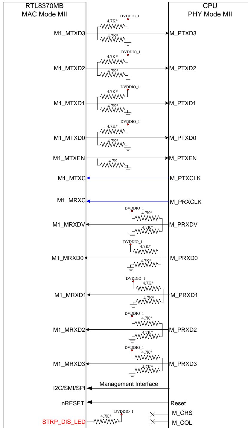
Figure 32. Signal Diagram of MII MAC Mode of the Extension GMAC1
