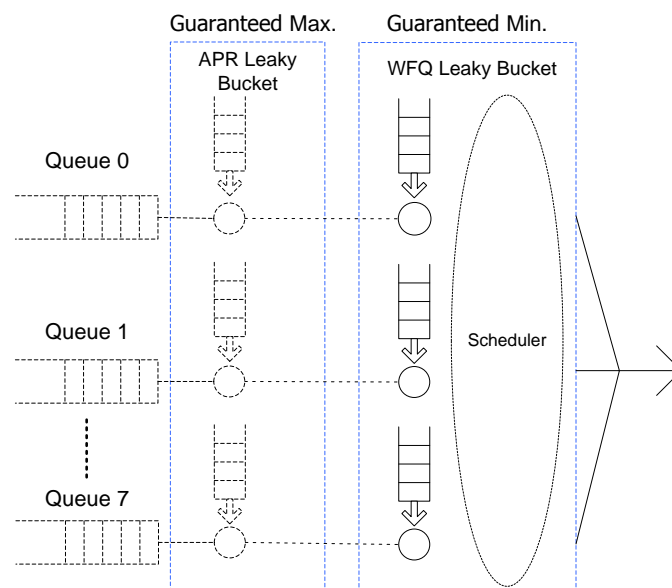
Figure 8. RTL8370MB MAX-MIN Scheduling Diagram
