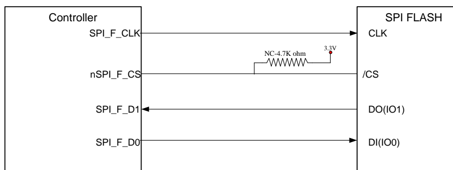
Figure 28. SPI FLASH Interface Connection Example
