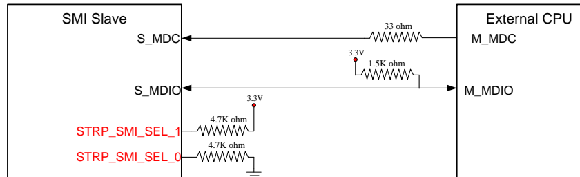
Figure 24. Slave MII Management SMI Interface Connection Example
