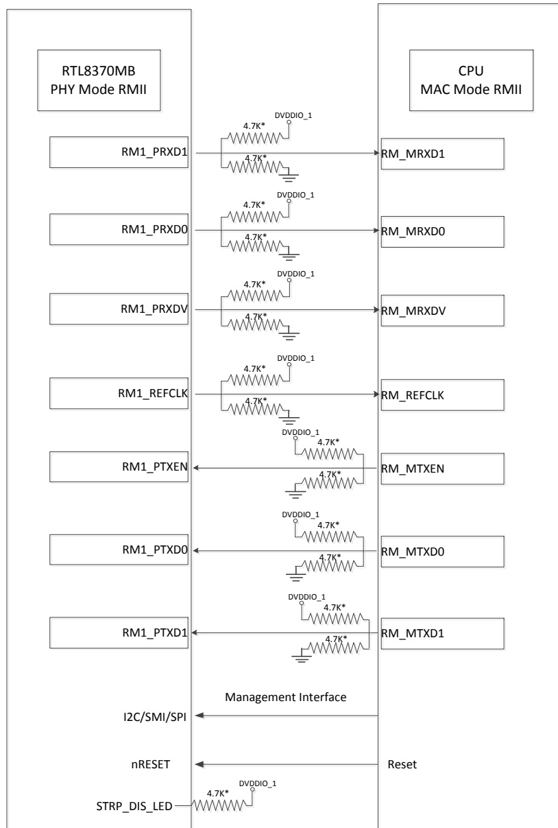
Figure 39. Signal Diagram of RMII PHY Mode of the Extension GMAC1
