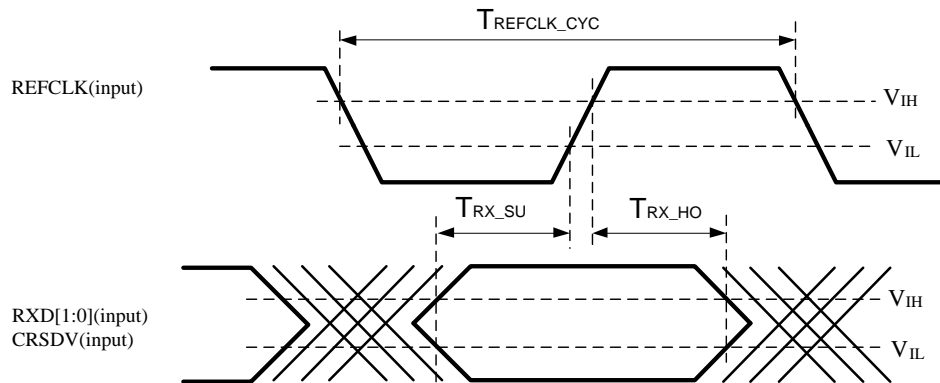
Figure 66. RMII MAC Mode Input Timing
