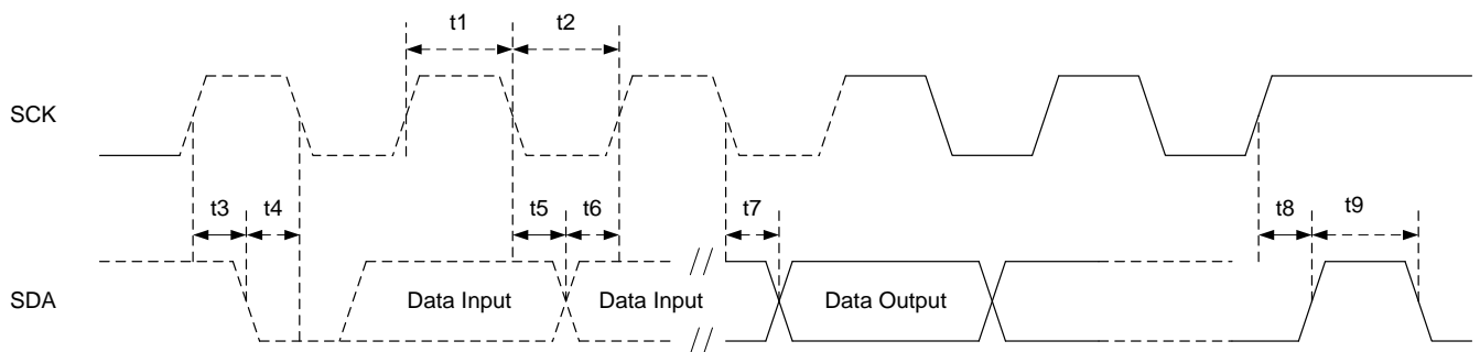
Figure 49. Slave I2C-Like for External CPU Access Interface Timing Characteristics
